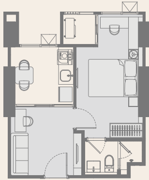
B1 | 31.00-31.50 sq.m.
