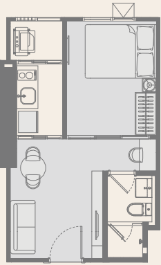
A1 | 27.20 sq.m.
